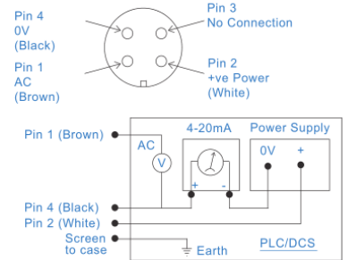
Connection Details
